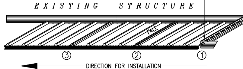
RIGHT HAND CUTBACK PANEL
