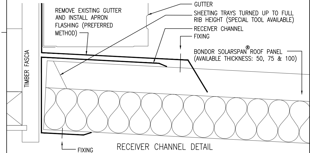
SOLARSPAN RECEIVER CHANNEL (VALID UP TO 7° ROOF PITCH)
