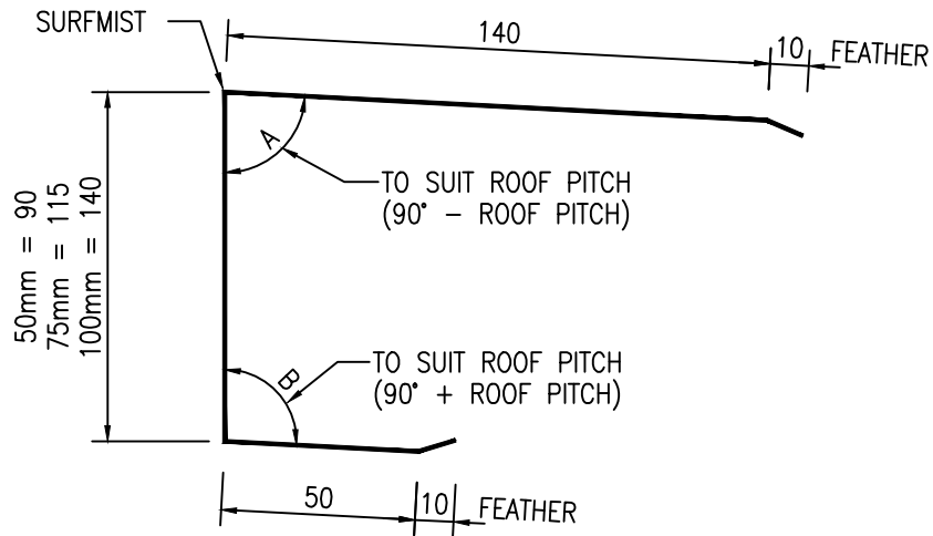
SOLARSPAN RECEIVER CHANNEL (VALID UP TO 7° ROOF PITCH)
